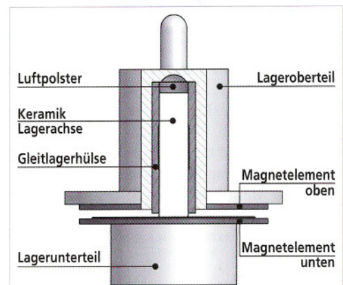
clearaudio CMB (ceramic magnetic bearing) Magnetlager
