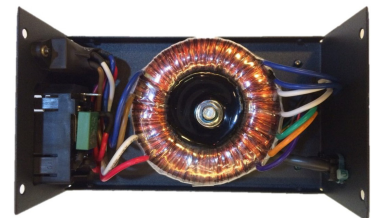
Toroidal Transformer
