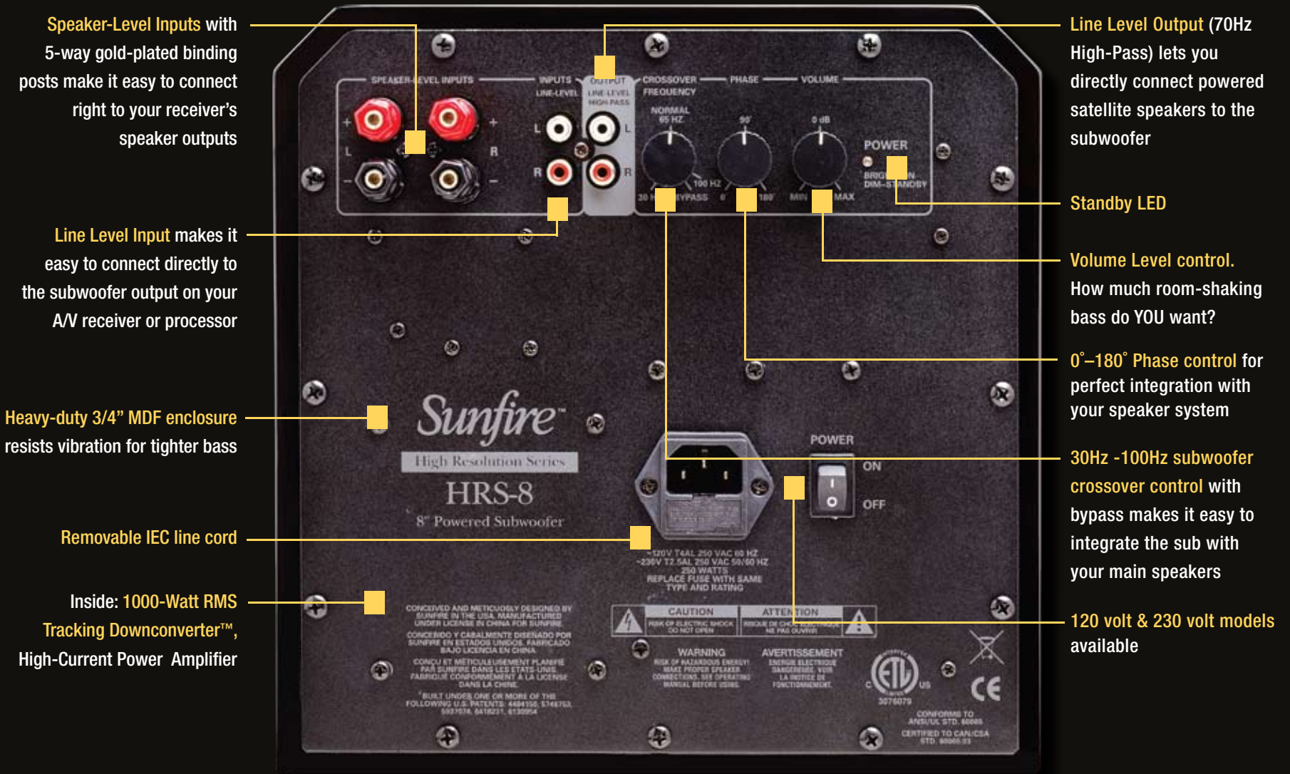
Back panel features identical on Models HRS-8, HRS-10 and HRS-12
