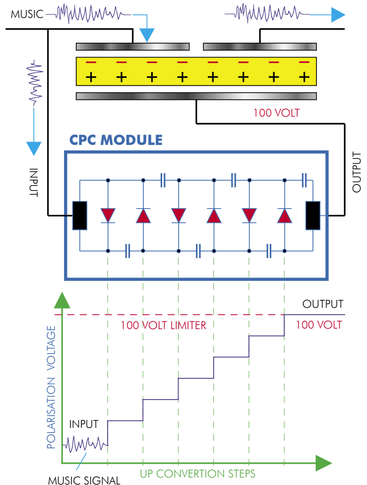
CPC UPCONVERSION OF MUSIC SIGNAL
