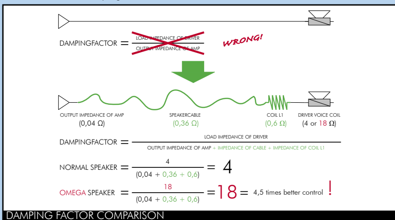
DAMPING FACTOR COMPARISON
