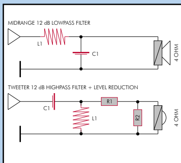
TYPICAL 12dB CROSSOVER
