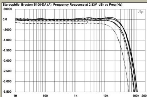
Fig.9 Bryston B100-DA, frequency response at 2.83V into (from top to bottom at 2kHz): simulated loudspeaker load, 8, 4, 2 ohms (0.5dB/vertical div.).
