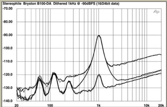
Fig.2 Bryston B100-DA, 1/2-octave spectrum with noise and spurious of dithered 1kHz tone at -90dBFS, 16-bit data (top) and 24-bit data (bottom). (Right channel dashed.)
