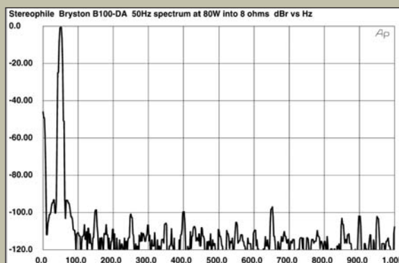
Fig.14 Bryston B100-DA, spectrum of 50Hz sinewave, DC–1kHz, at 80W into 8 ohms (linear frequency scale).
