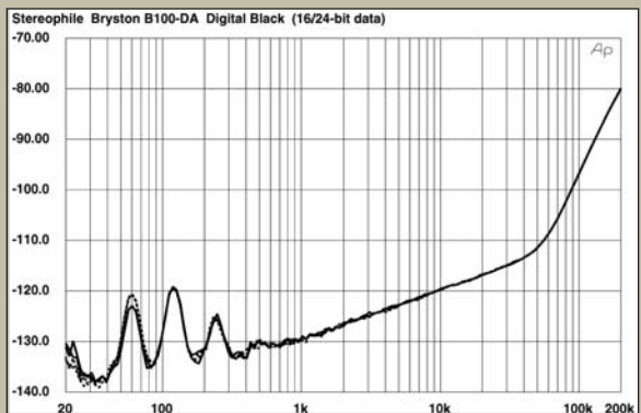
Fig.3 Bryston B100-DA, 1/2-octave spectrum with noise and spurious of digital black, 24-bit data (right channel dashed).
