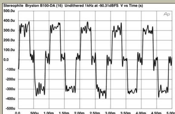
Fig.5 Bryston B100-DA, waveform of undithered 1kHz sinewave at -90.31dBFS, 16-bit data.
