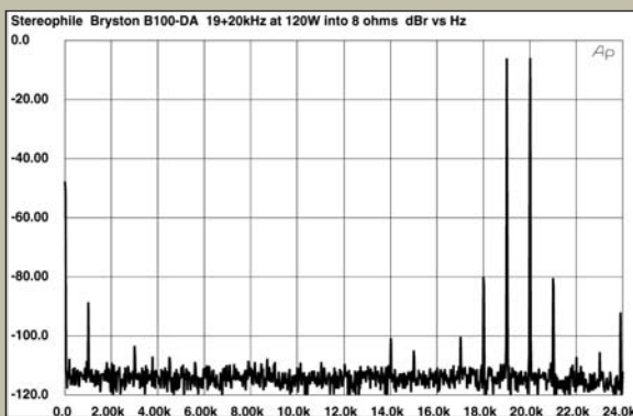
Fig.15 Bryston B100-DA, HF intermodulation spectrum, DC–24kHz, 19+20kHz at 120W peak into 8 ohms (linear frequency scale).
