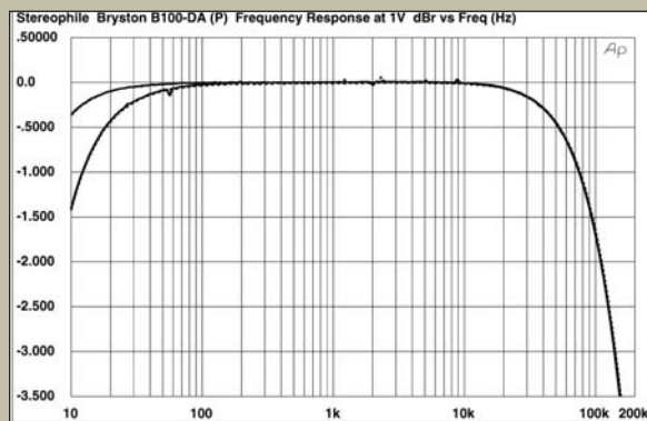
Fig.7 Bryston B100-DA, preamplifier frequency response at 1V into (from top to bottom at 20Hz): 100k, 600 ohms (0.5dB/vertical div., right channel dashed).
